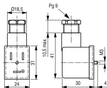
Conector Retangular
